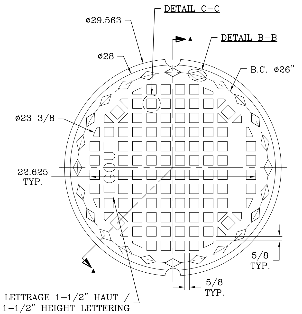
TOP VIEW
